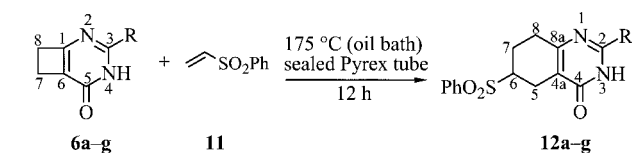
Scheme 2. Regioselective Diels–Alder reactions of phenyl vinyl sulfone ( 11 ) with the cyclobutene-annulated pyrimidinones 6a–g . For details see Table 2.
