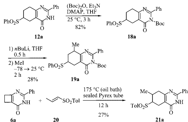
Scheme 5. Alkylation of the N -Boc-protected 18a at C-8 and preparation of a 7-substituted tetrahydroquinazolinone 21a .
