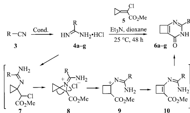
Scheme 1. Michael addition of amidines 4 to methyl 2-chloro-2-cyclopropylideneacetate ( 5 ) to yield cyclobutene-annulated pyrimidinones 6 . Conditions A : LiN(SiMe 3 ) 2 (1 M, THF), THF, 25 °C, 4 h; conditions B : Me 3 Al (2 M, toluene), NH 4 Cl, toluene, 120 °C, 20 h (for further details see Table 1).
