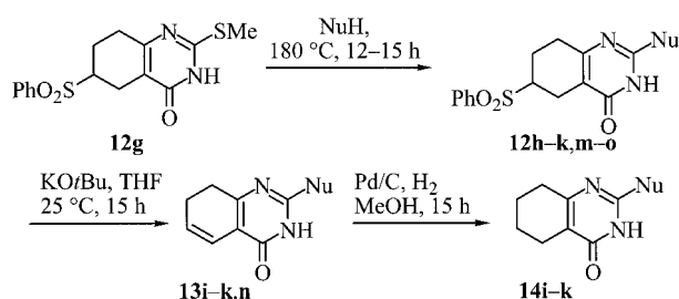
Scheme 6. Nucleophilic substitution of the methylthio group in 12g by amines. For details see Table 4.
