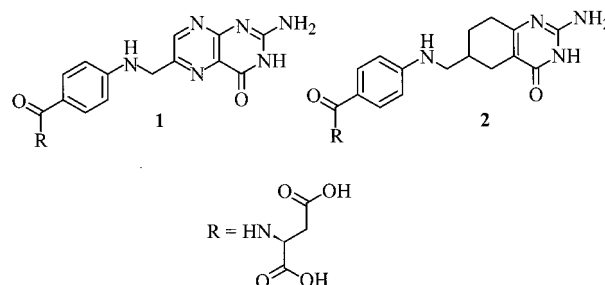
Figure 1. Coenzyme folic acid ( 1 ) and its dideazatetrahydro analogue 2 .
