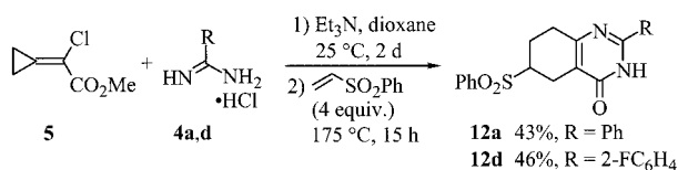
Scheme 3. One-pot, two-step synthesis of tetrahydroquinazolinones 12a,d from 5 , amidines 4a,d and phenyl vinyl sulfone ( 11 ).
