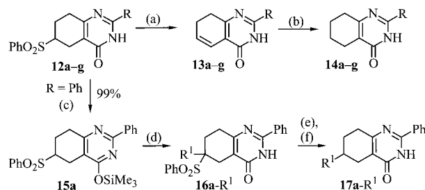
Scheme 4. Preparation of 2-substituted and 2,6-disubstituted tetrahydroquinazolinones: (a) KO t Bu (3 equiv.), THF, 25 °C, 2 h; (b) Pd/C (10% Pd, w/w), H 2 , MeOH or AcOH, 25 °C, 4–8 h; (c) HN(SiMe 3 ) 2 , (NH 4 ) 2 SO 4 , 126 °C, 15 h; (d) n BuLi, THF, –78 °C, 30 min, then MeI or EtBr, 25 °C, 2 h; (e) KO t Bu, THF, 25 °C, 2 h; (f) Pd/C, H 2 , MeOH, 25 °C, 4 h. For further details see Table 3.
